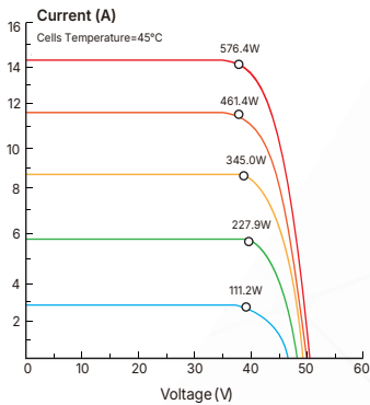
Current-Voltage Curve(610W)
