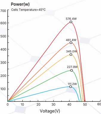
Power-Voltage Curve(610W)
